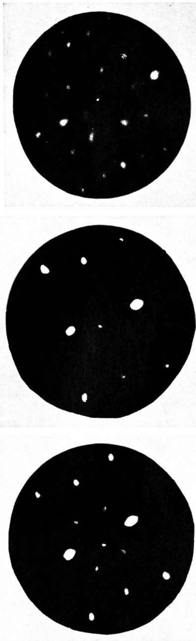
Fig. 7. LEED patterns of oxygen covered Ir(110) surfaces. a) 2 \times 2 -structure, b) 1 \times 1 -structure after interaction with O_2 at 400^\circ C , c) c2 \times 2 -structure after cooling in O_2 atmosphere.
