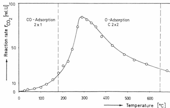
Fig. 8. Steady-state rate of CO 2 formation in a CO/O 3 mixture as a function of temperature.
